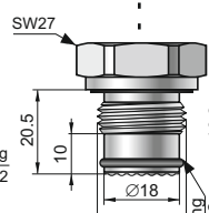
G1/2 type G1/2", Ø4 hole M type M20×1.5, Ø4 hole
