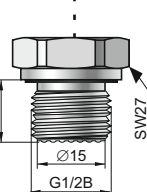
CG1/2 type G1/2" with flush diaphragm
