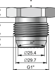
CG1-S38 type G1" with flush diaphragm
